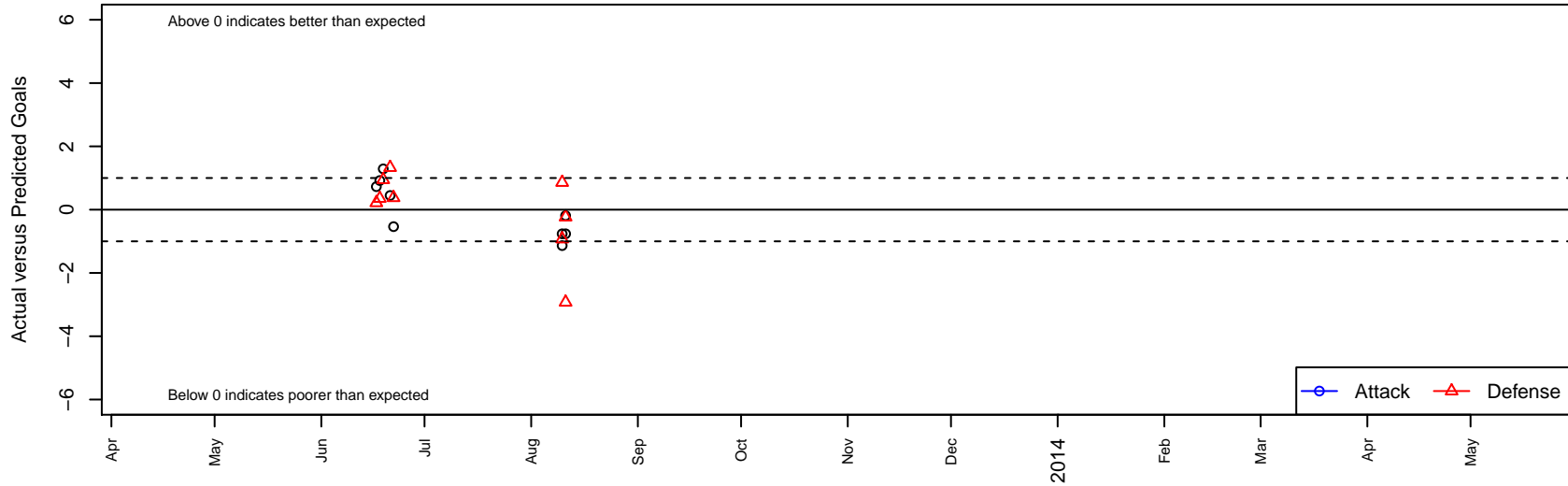
Las Vegas Premier Black B95 Dots are actual minus expected GF (blue circles) and GA (red triangles). Blue line is smoothed change in attack strength. Red is smoothed change in defense strength.
